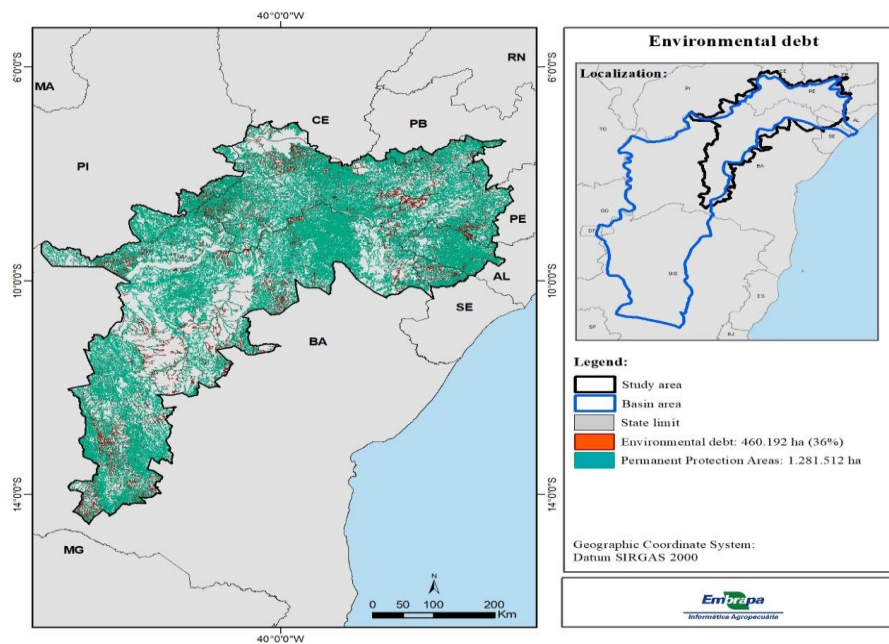
Figure 5: Environmental debt in some municipalities of Caatinga inside Basin of São Francisco (Pugliero, et al 2018)
