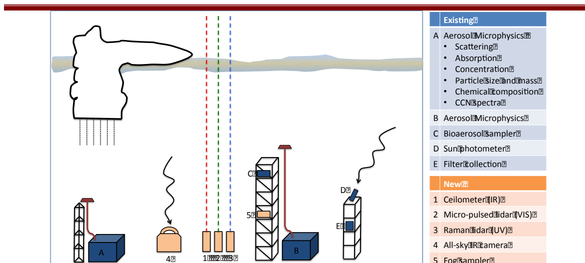
Figure 19 – Schematic view of the aerosol measurements at the ATTO site. Detailed aerosol particle microphysics measurements are already in operation at the 60 m triangular tower (A), and the 325 meters tall tower (B). Filter collection for elemental chemical composition, and organic and elemental carbon concentration (E) takes place at the walkup tower, and for analysis of fungi and spores (C), at the tall tower. New instruments will allow measuring the vertical profile of aerosol and cloud properties.
